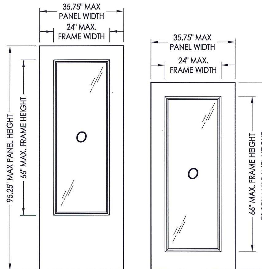
SMART FRAME DOORGLASS ASSEMBLY
