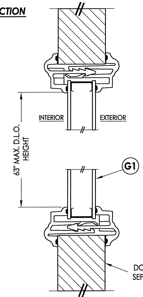
1 2 VERTICAL CROSS SECTION
